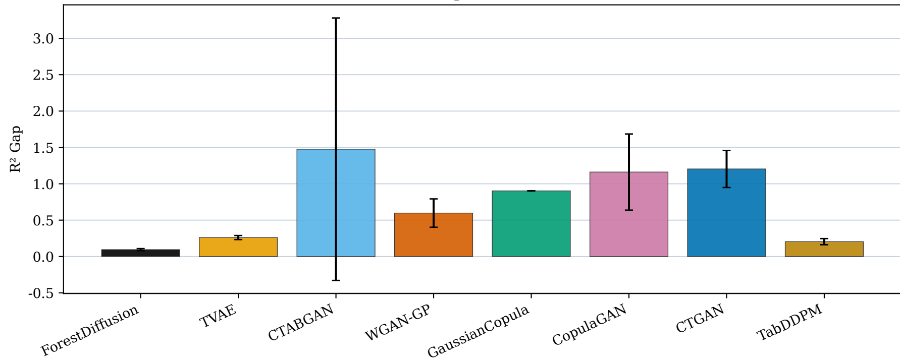
Concrete — R^2 Gap (mean \pm SD, 10 seeds)
